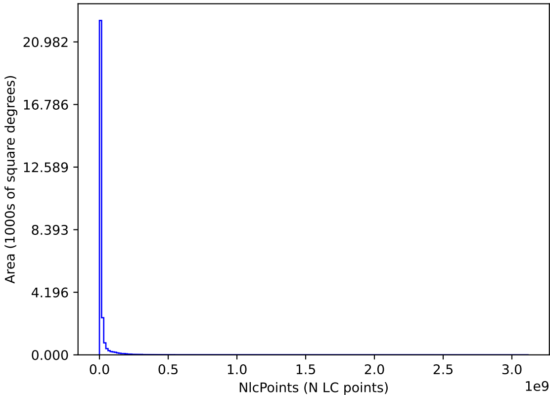
too_elab_r8_d2_gz_v3.4_10yrs : NlcPoints
