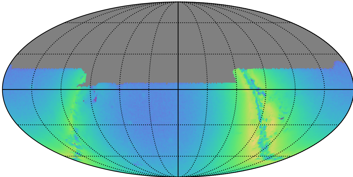
too_elab_r8_d2_gz_v3.4_10yrs u: N stars to Precision 0.20
