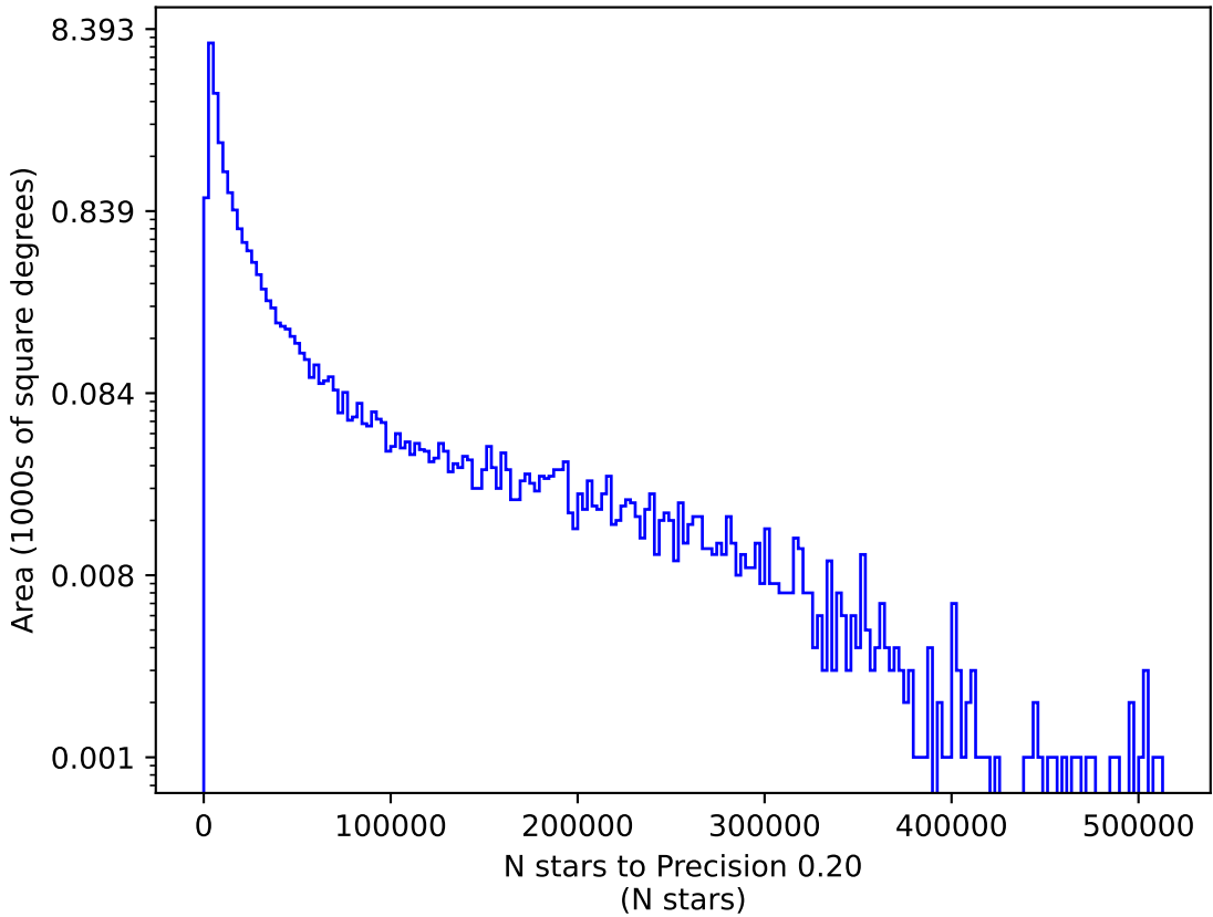
too_elab_r8_d2_gz_v3.4_10yrs u: N stars to Precision 0.20
