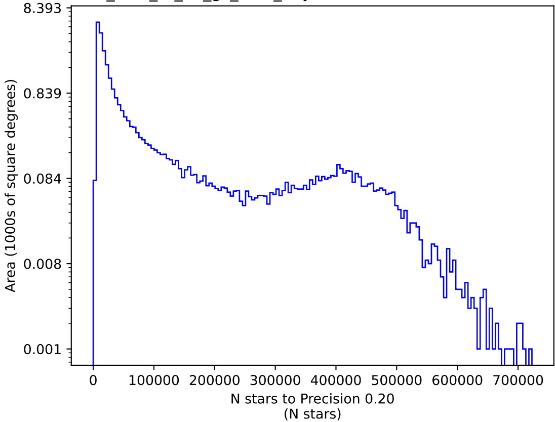
too_elab_r8_d2_gz_v3.4_10yrs i: N stars to Precision 0.20
