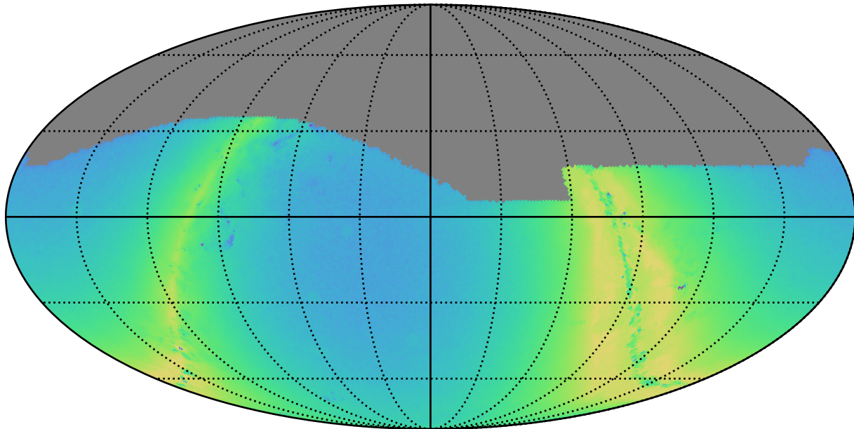
too_elab_r8_d2_gz_v3.4_10yrs g: N stars to Precision 0.20
