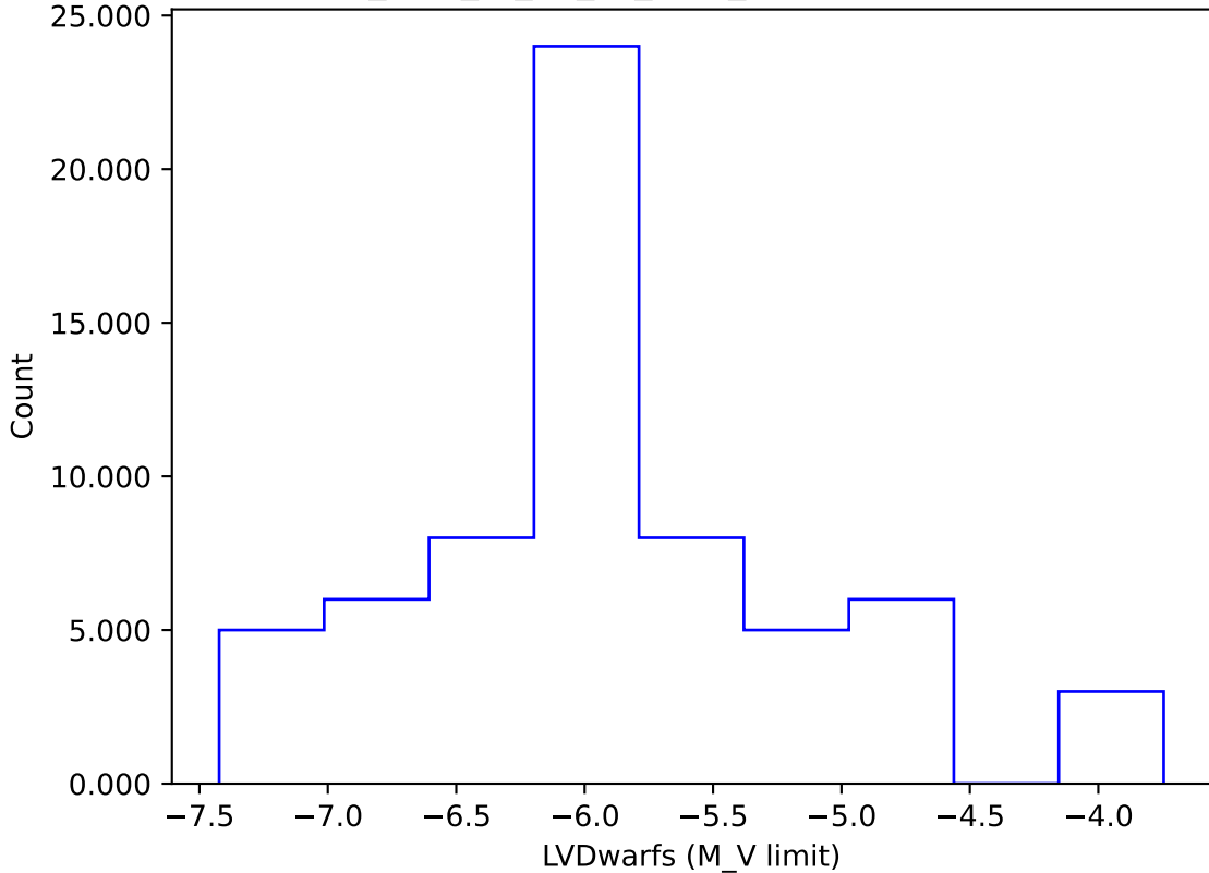
too_elab_r8_d2_gz_v3.4_10yrs gi: LVDwarfs
