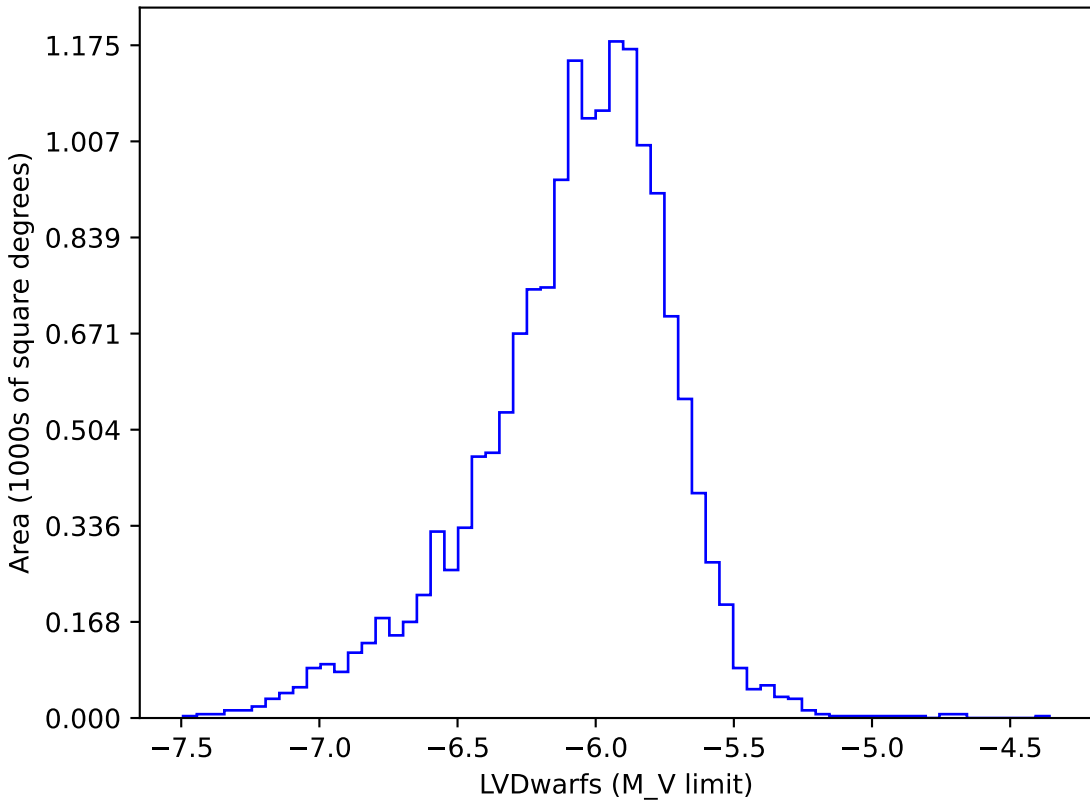
too_elab_r8_d2_gz_v3.4_10yrs gi: LVDwarfs
