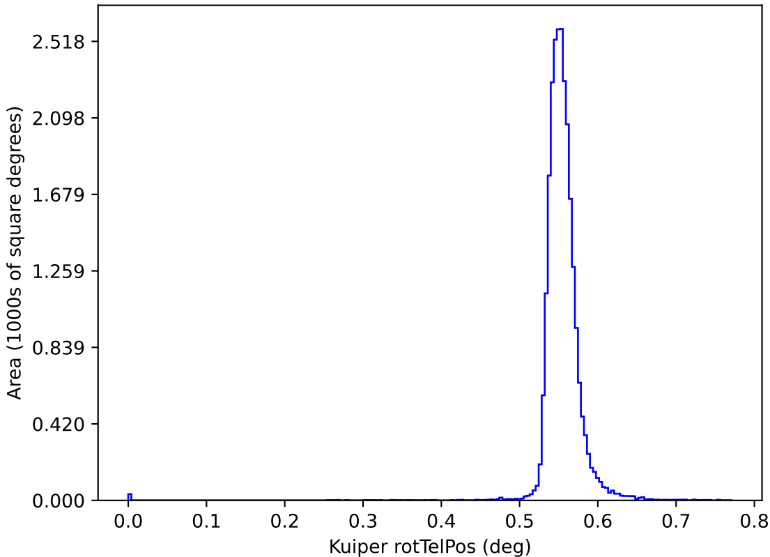
too_elab_r8_d2_gz_v3.4_10yrs y: Kuiper rotTelPos
