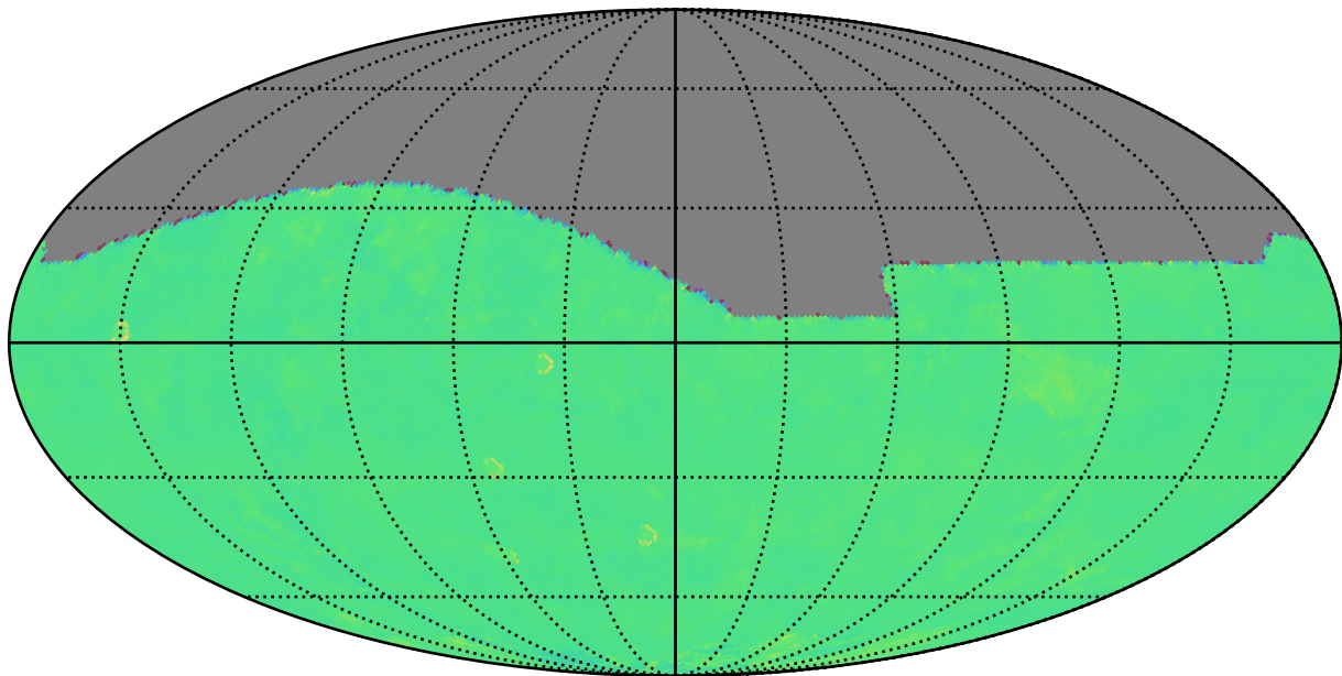
too_elab_r8_d2_gz_v3.4_10yrs r: Kuiper rotTelPos
