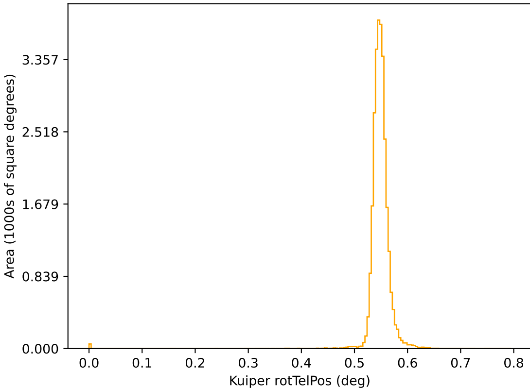
too_elab_r8_d2_gz_v3.4_10yrs r: Kuiper rotTelPos
