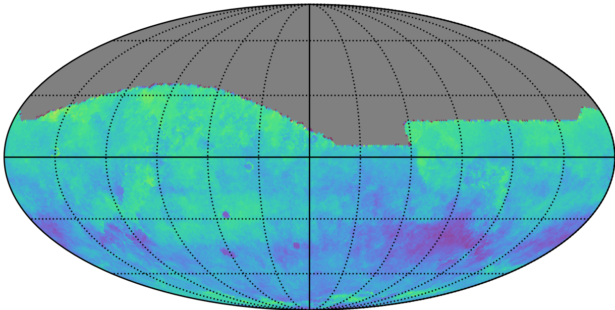
too_elab_r8_d2_gz_v3.4_10yrs z: Kuiper rotSkyPos
