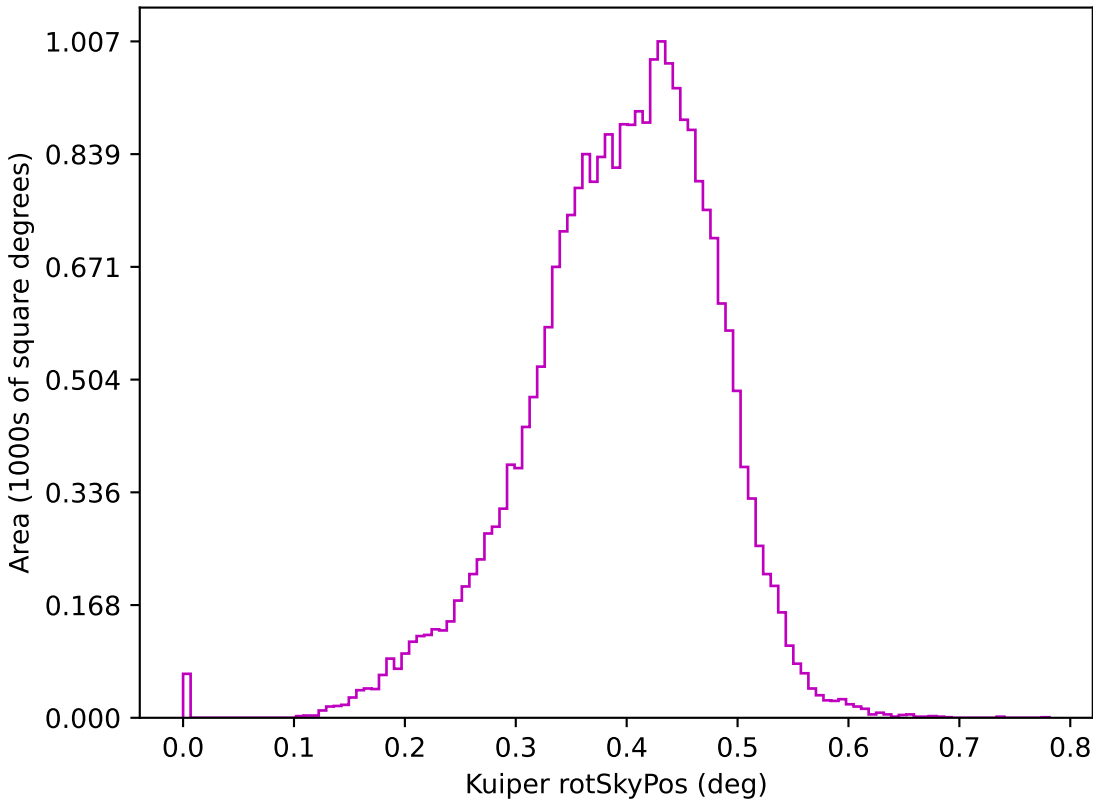
too_elab_r8_d2_gz_v3.4_10yrs z: Kuiper rotSkyPos
