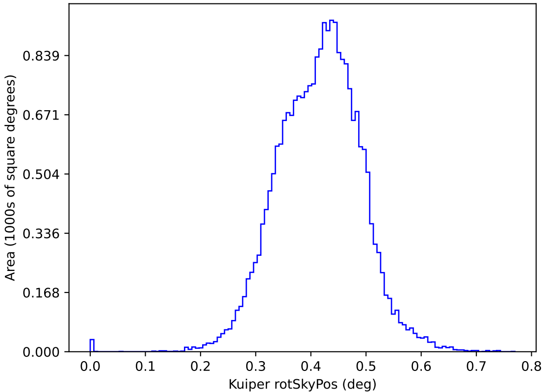
too_elab_r8_d2_gz_v3.4_10yrs y: Kuiper rotSkyPos
