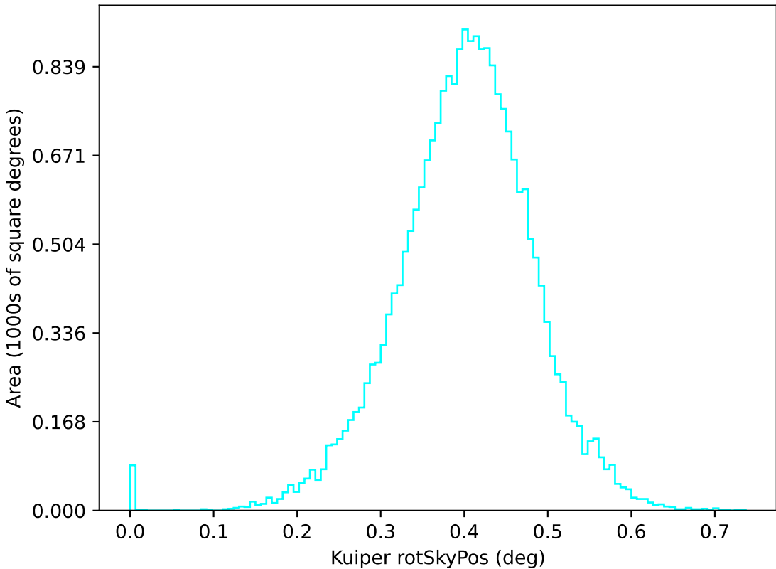
too_elab_r8_d2_gz_v3.4_10yrs u: Kuiper rotSkyPos
