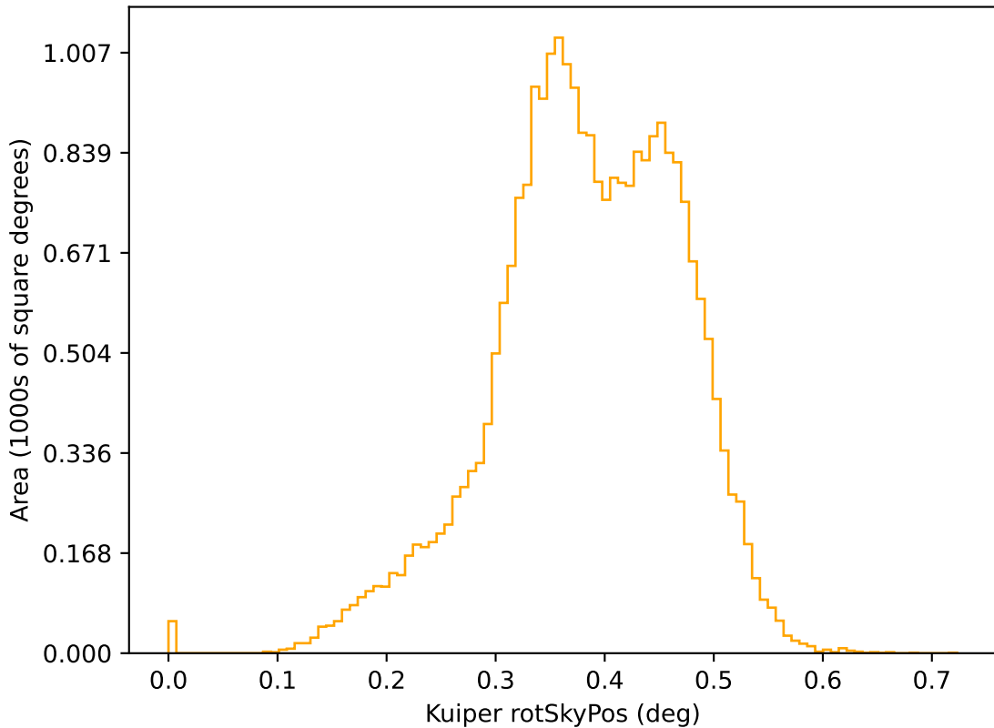
too_elab_r8_d2_gz_v3.4_10yrs r: Kuiper rotSkyPos
