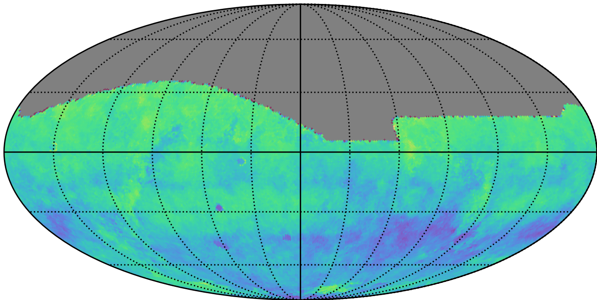
too_elab_r8_d2_gz_v3.4_10yrs i: Kuiper rotSkyPos
