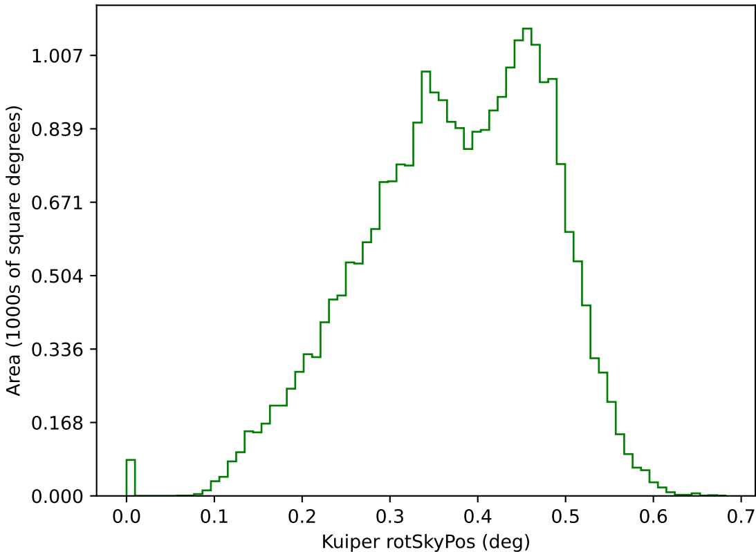
too_elab_r8_d2_gz_v3.4_10yrs g: Kuiper rotSkyPos
