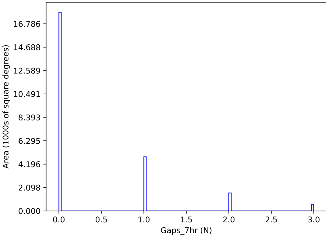
too_elab_r8_d2_gz_v3.4_10yrs y band: Gaps_7hr
