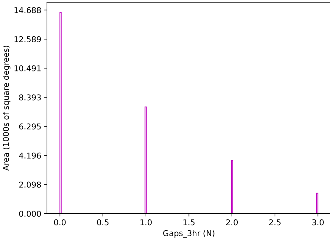
too_elab_r8_d2_gz_v3.4_10yrs z band: Gaps_3hr
