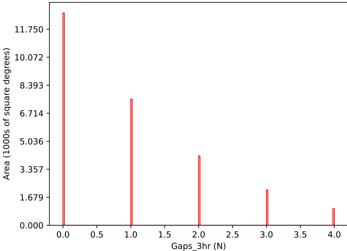
too_elab_r8_d2_gz_v3.4_10yrs i band: Gaps_3hr
