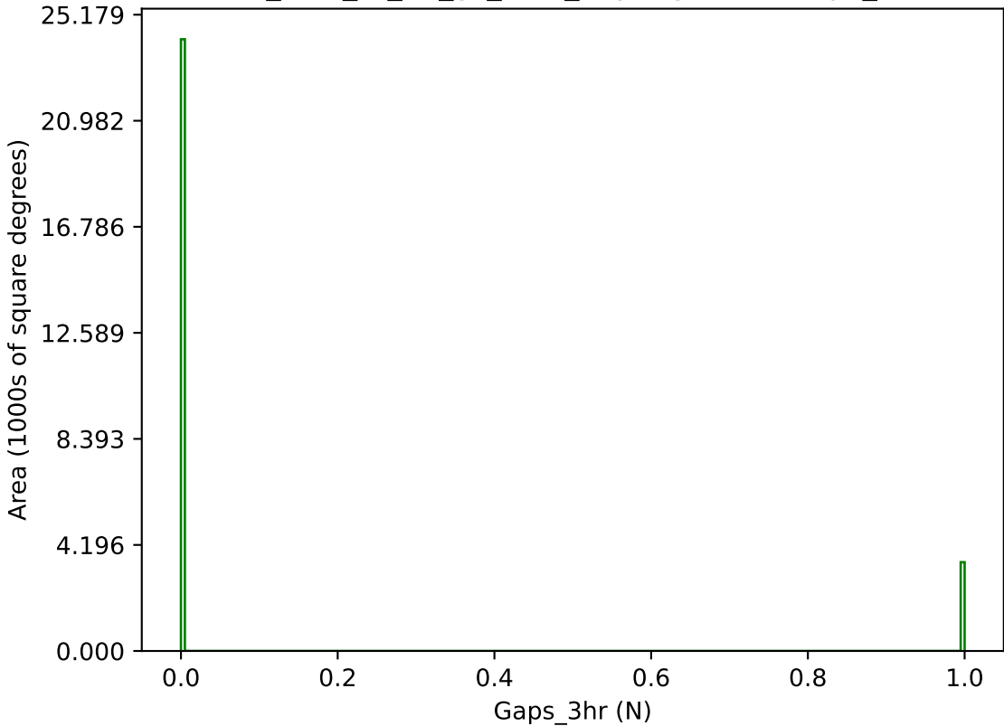
too_elab_r8_d2_gz_v3.4_10yrs g band: Gaps_3hr
