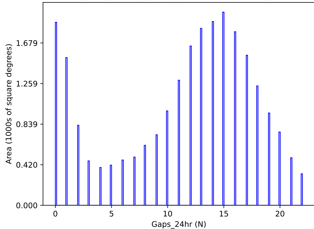
too_elab_r8_d2_gz_v3.4_10yrs y band: Gaps_24hr
