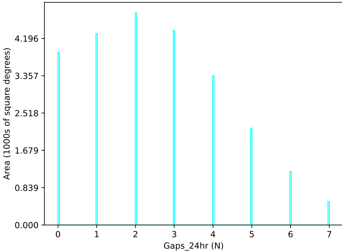
too_elab_r8_d2_gz_v3.4_10yrs u band: Gaps_24hr
