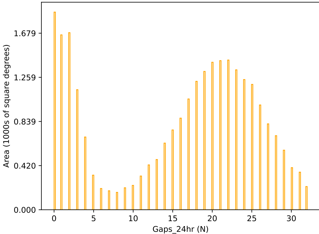
too_elab_r8_d2_gz_v3.4_10yrs r band: Gaps_24hr
