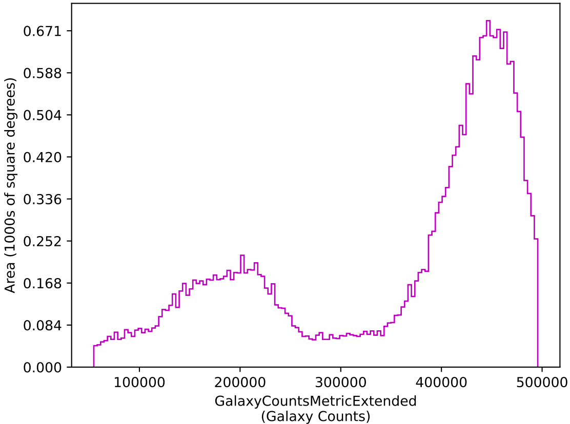
too_elab_r8_d2_gz_v3.4_10yrs z: GalaxyCountsMetricExtended
