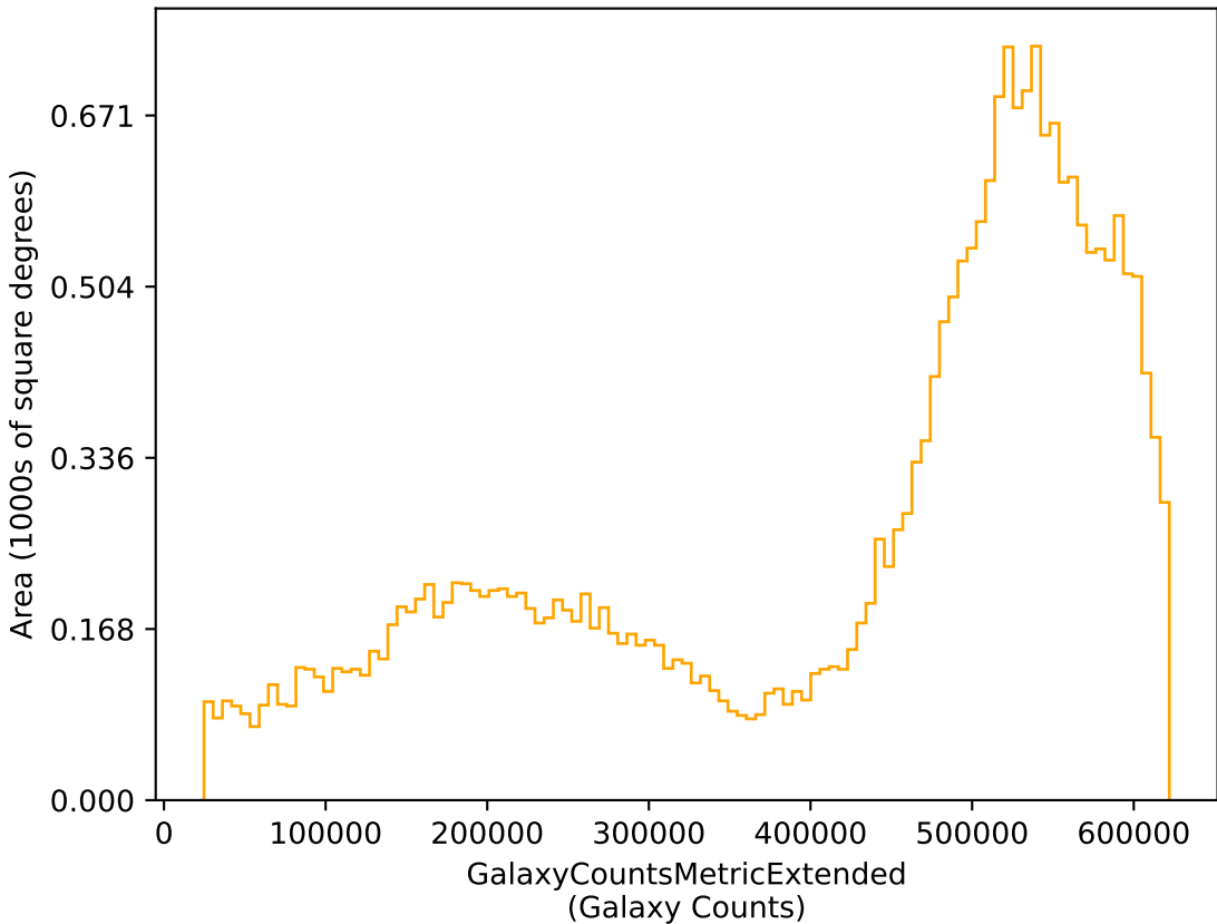
too_elab_r8_d2_gz_v3.4_10yrs r: GalaxyCountsMetricExtended
