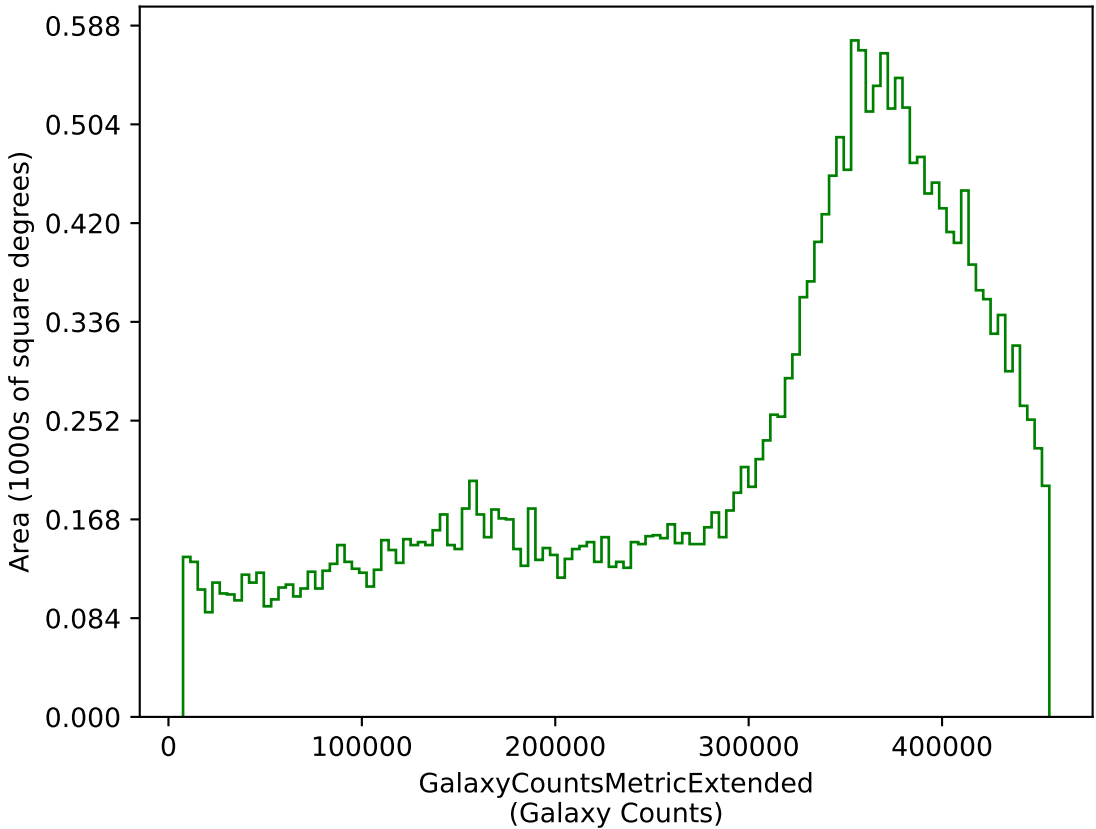
too_elab_r8_d2_gz_v3.4_10yrs g: GalaxyCountsMetricExtended
