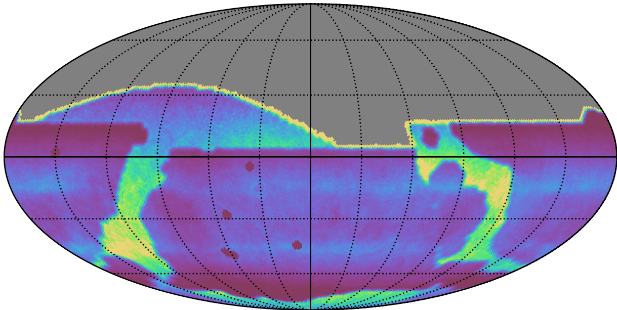
too_elab_r8_d2_gz_v3.4_10yrs : DCRprecision
