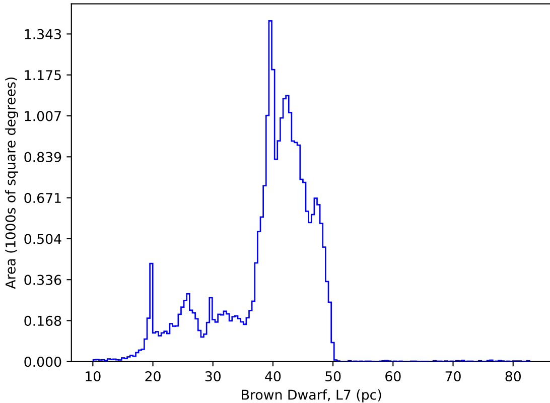
too_elab_r8_d2_gz_v3.4_10yrs : Brown Dwarf, L7
