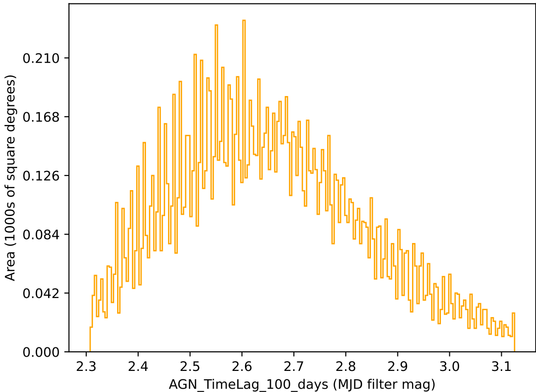
too_elab_r8_d2_gz_v3.4_10yrs r band: AGN_TimeLag_100_days
