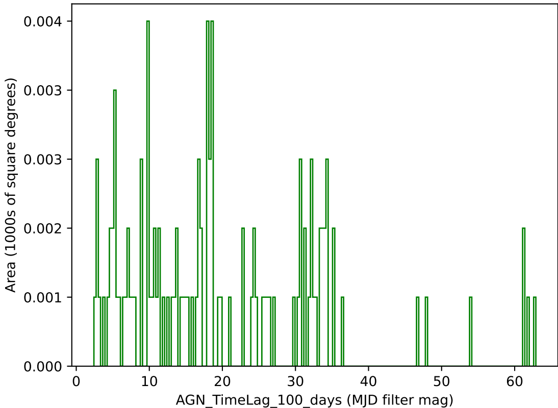
too_elab_r8_d2_gz_v3.4_10yrs g band: AGN_TimeLag_100_days
