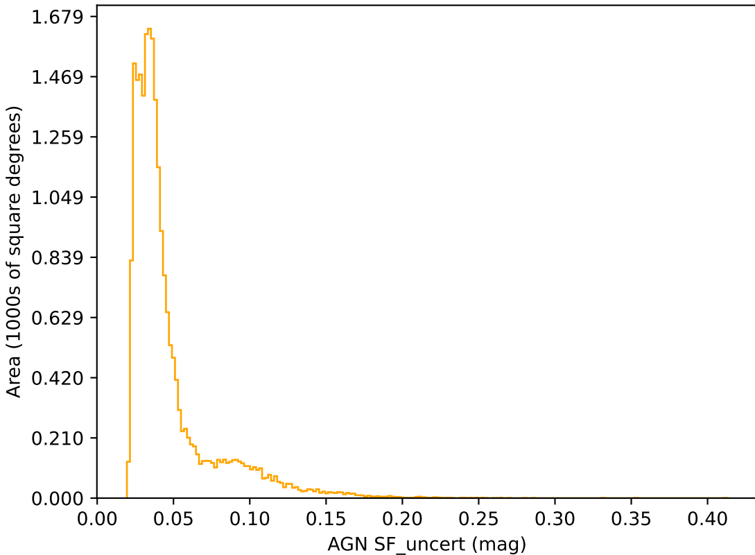
too_elab_r8_d2_gz_v3.4_10yrs r band: AGN SF_uncert
