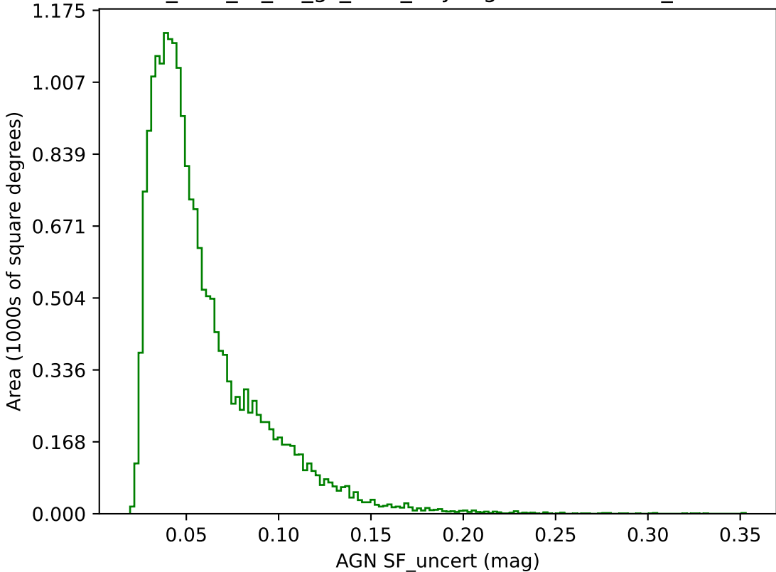
too_elab_r8_d2_gz_v3.4_10yrs g band: AGN SF_uncert
