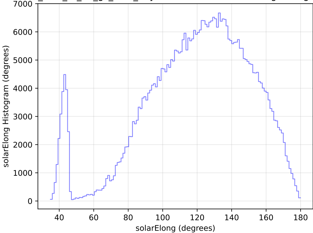
too_elab_r8_d2_gz_v3.4_10yrs WFD z band: solarElong Histogram
