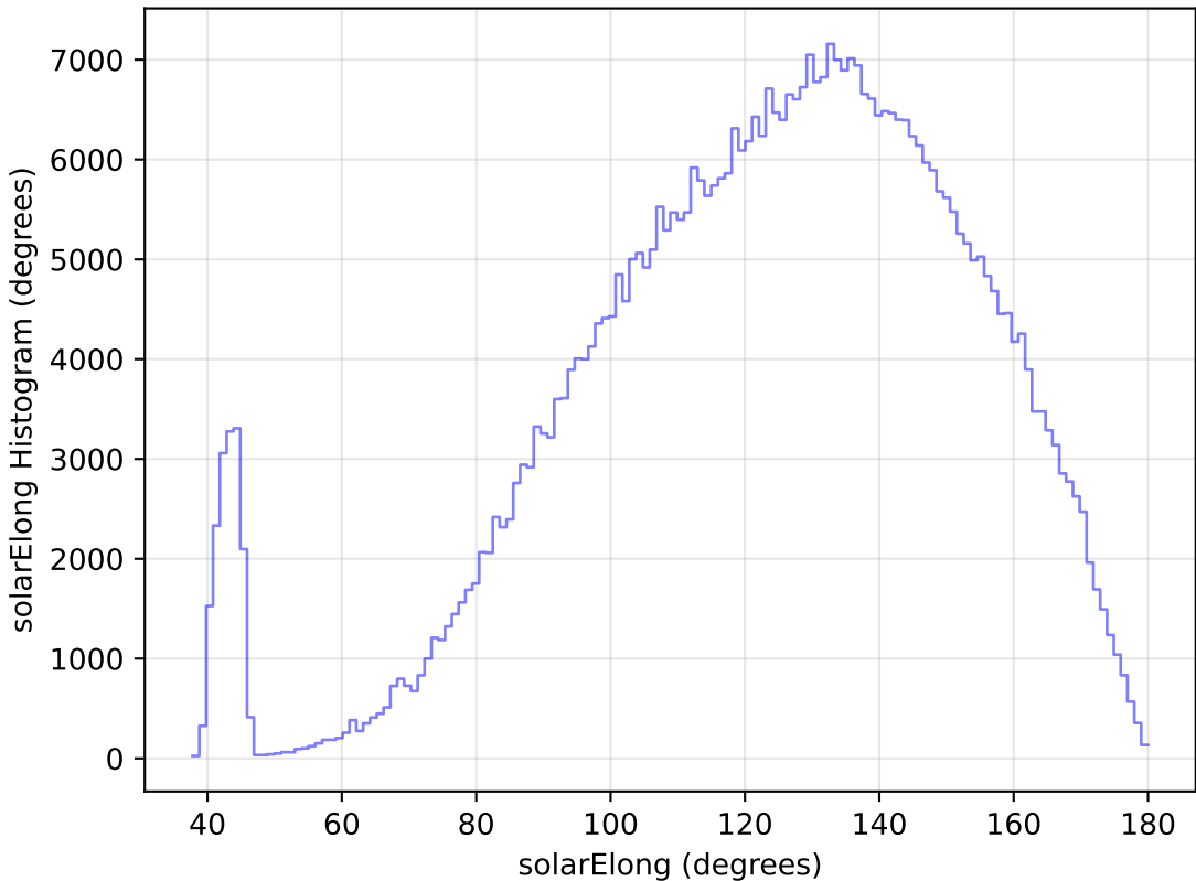
too_elab_r8_d2_gz_v3.4_10yrs WFD r band: solarElong Histogram
