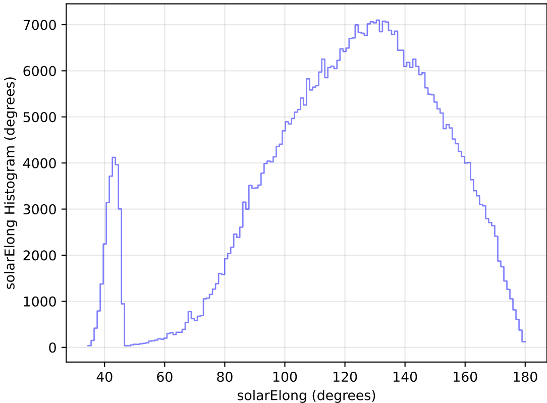
too_elab_r8_d2_gz_v3.4_10yrs WFD i band: solarElong Histogram
