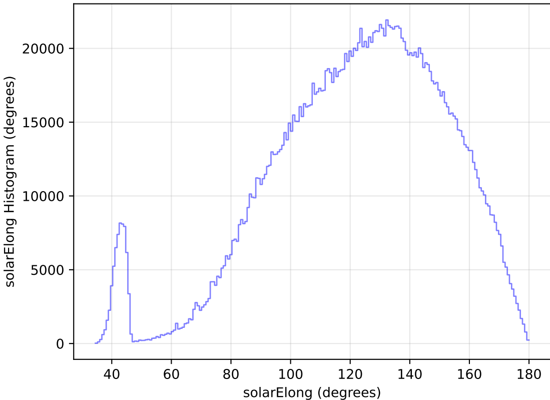
too_elab_r8_d2_gz_v3.4_10yrs WFD all bands: solarElong Histogram
