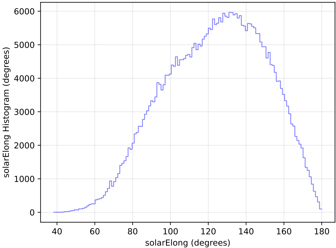
too_elab_r8_d2_gz_v3.4_10yrs All sky y band: solarElong Histogram
