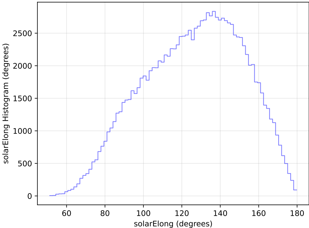
too_elab_r8_d2_gz_v3.4_10yrs All sky u band: solarElong Histogram
