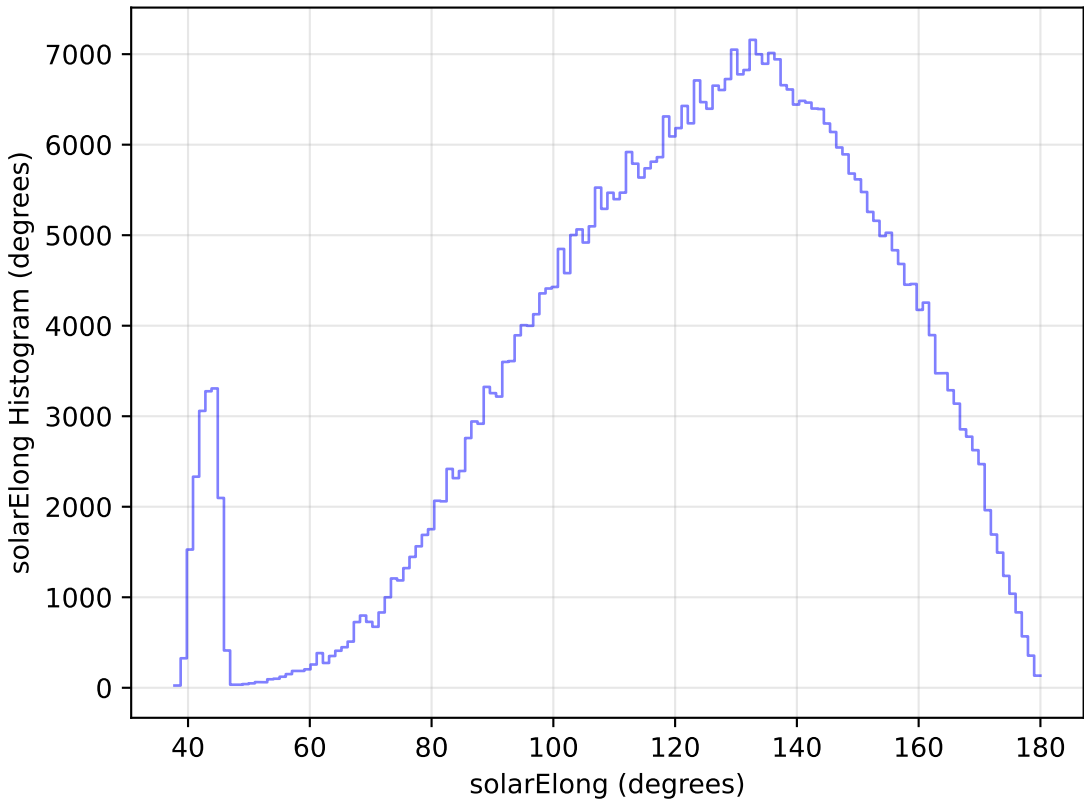
too_elab_r8_d2_gz_v3.4_10yrs All sky r band: solarElong Histogram
