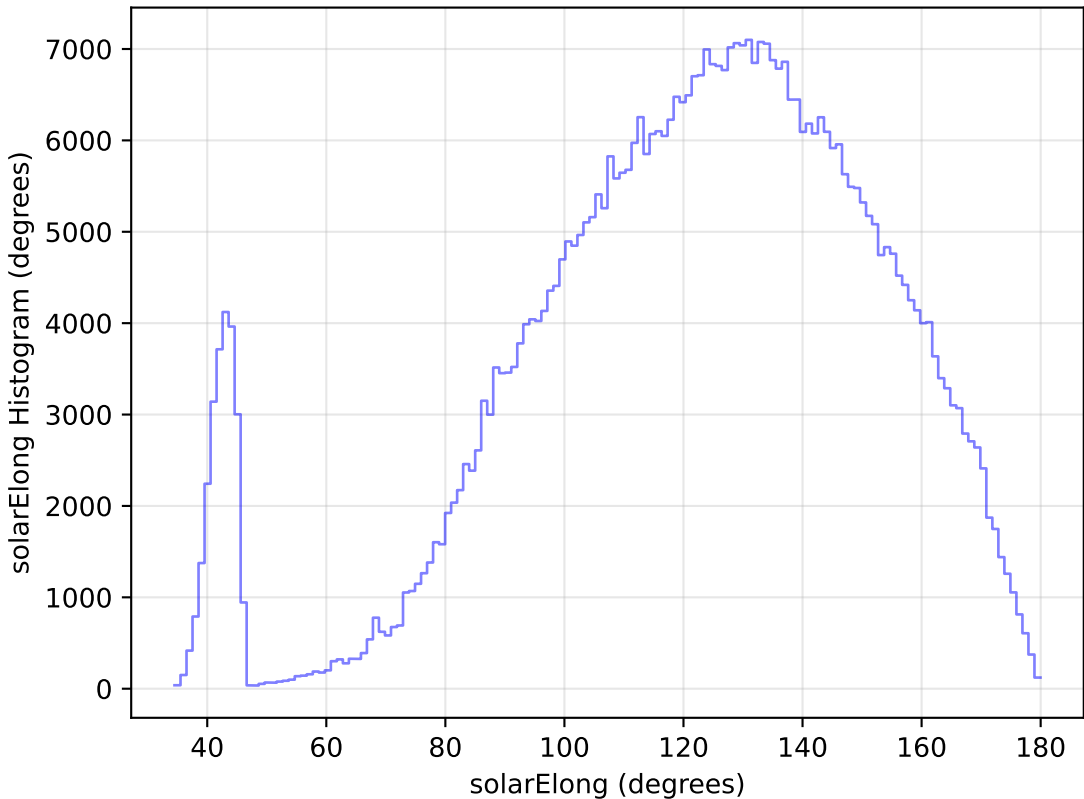
too_elab_r8_d2_gz_v3.4_10yrs All sky i band: solarElong Histogram
