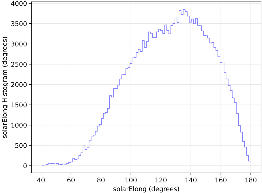
too_elab_r8_d2_gz_v3.4_10yrs All sky g band: solarElong Histogram
