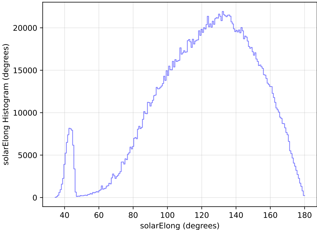
too_elab_r8_d2_gz_v3.4_10yrs All sky all bands: solarElong Histogram
