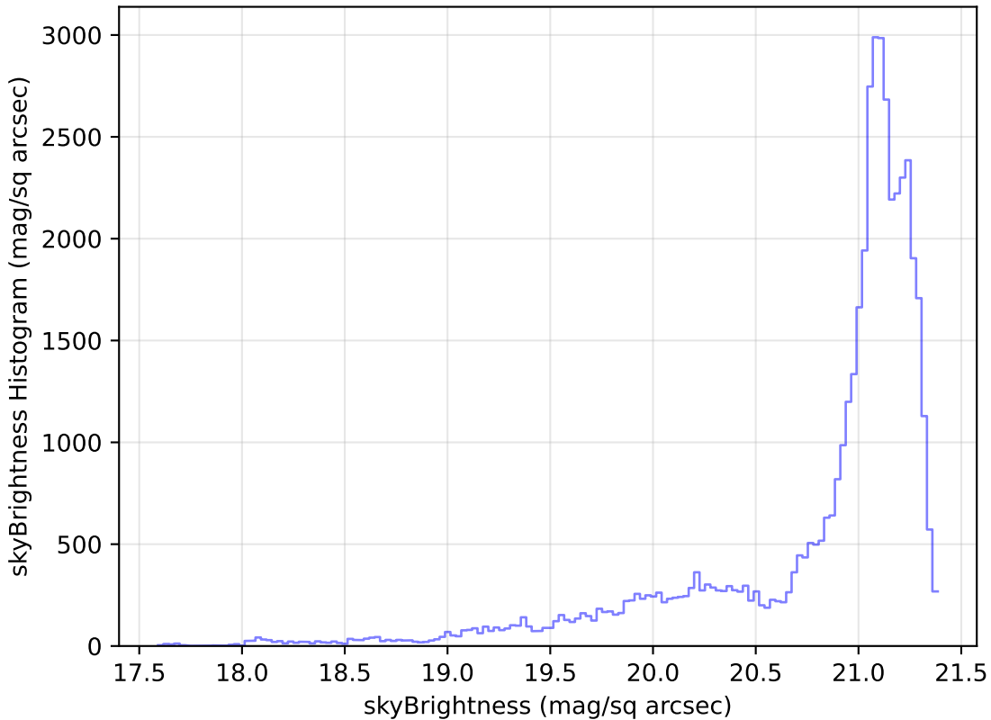
too_elab_r8_d2_gz_v3.4_10yrs Yr 1 r band: skyBrightness Histogram
