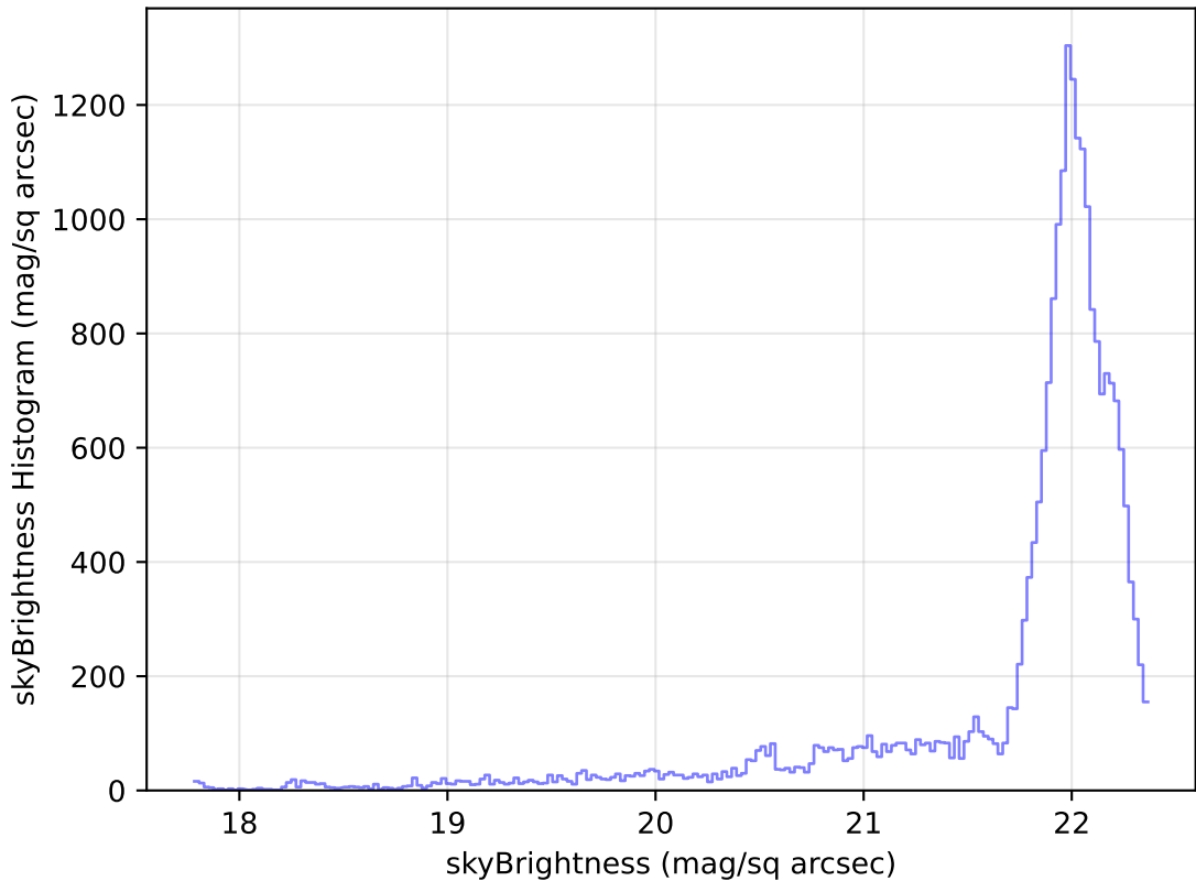
too_elab_r8_d2_gz_v3.4_10yrs Yr 1 g band: skyBrightness Histogram
