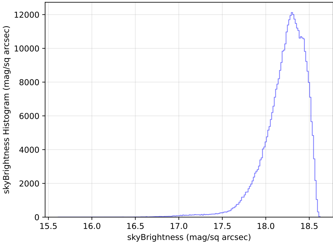
too_elab_r8_d2_gz_v3.4_10yrs WFD y band: skyBrightness Histogram
