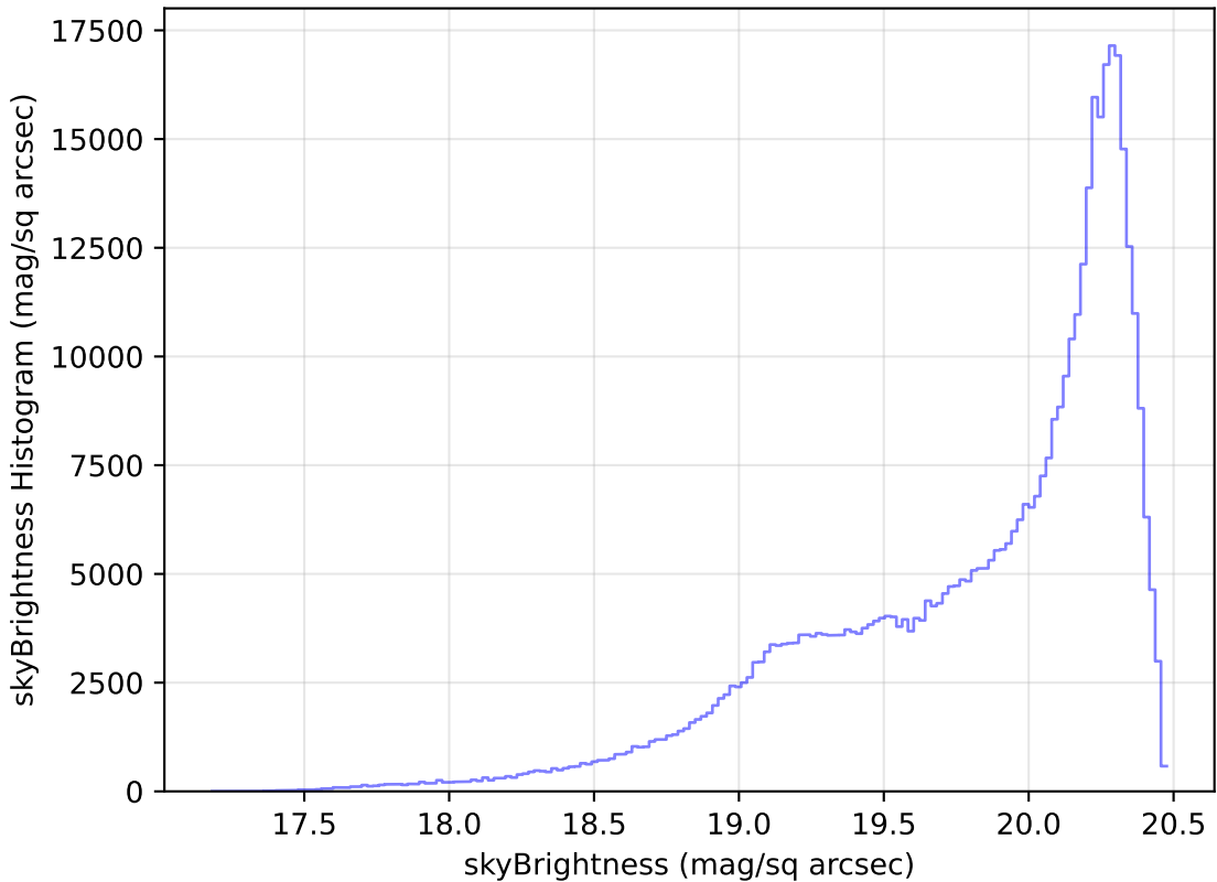
too_elab_r8_d2_gz_v3.4_10yrs WFD i band: skyBrightness Histogram
