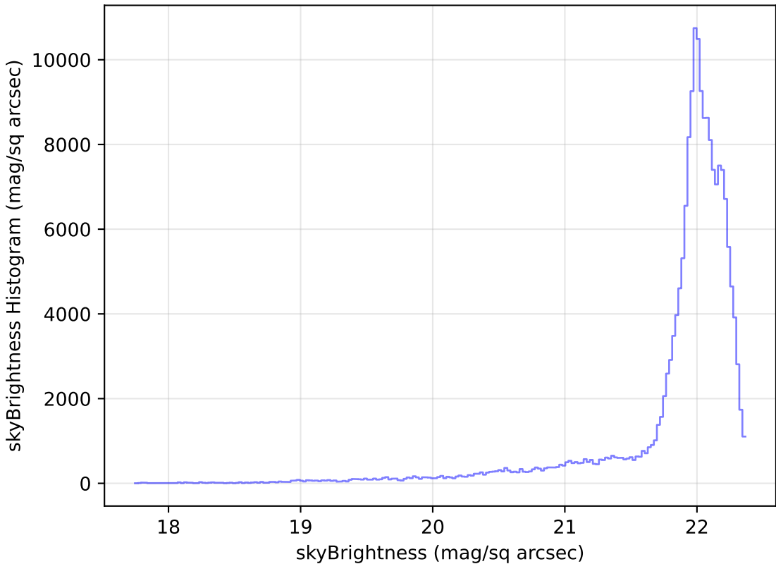
too_elab_r8_d2_gz_v3.4_10yrs WFD g band: skyBrightness Histogram
