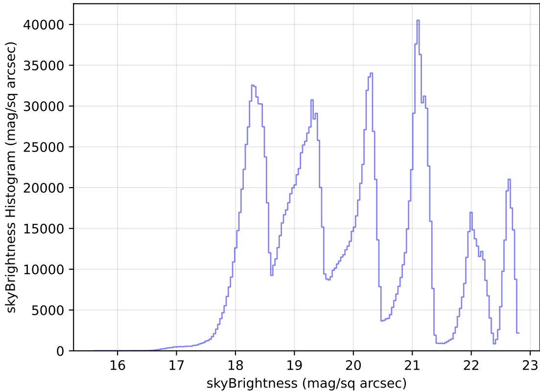
too_elab_r8_d2_gz_v3.4_10yrs WFD all bands: skyBrightness Histogram
