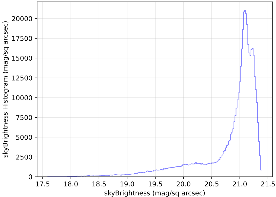
too_elab_r8_d2_gz_v3.4_10yrs All sky r band: skyBrightness Histogram
